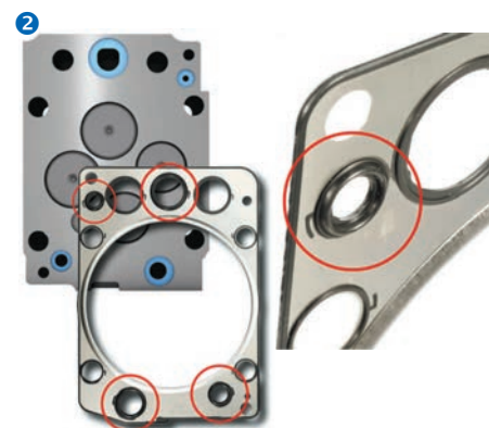
3 mm higher rubber sealing lip
